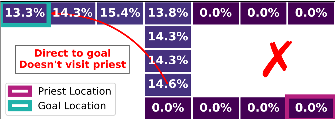
Fully-Observable Expert
