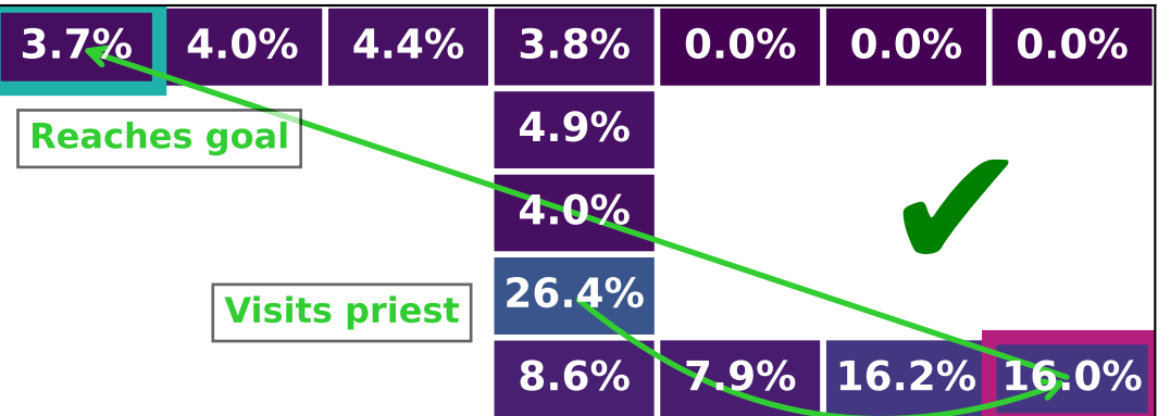
CO-CQL
