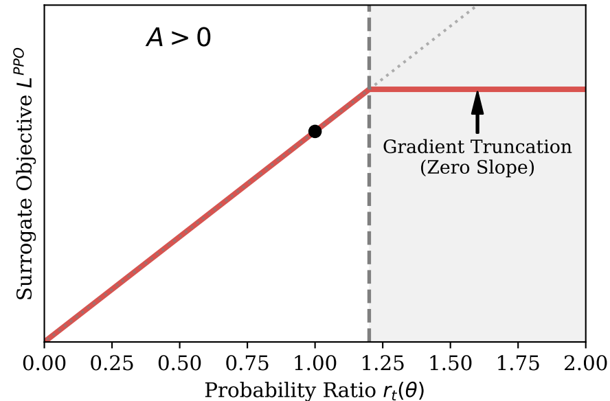
MAPPO (Symmetric Additive Clipping)
