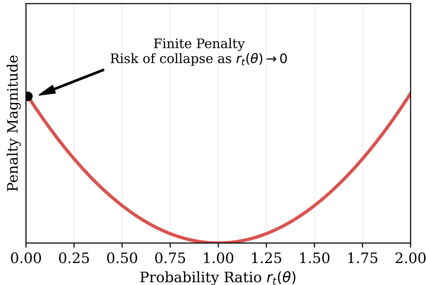
MASPO (Soft Quadratic Penalty)
